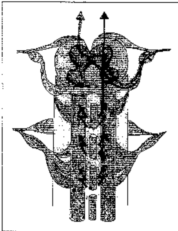
Fig 3. —Mode of action of spinal cord stimulation. Antidromic excitation of low-threshold fibers in dorsal columns is believed to activate inhibitory circuits in the dorsal horn. The simultaneous orthodromic activation of dorsal columns may activate supraspinal-gating mechanisms. 11
